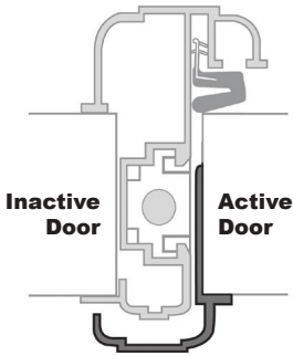
Add on an Astragal Security Strip to any outswing double door combination for added security and clean finished appearance eliminating the reveal between the doors.
